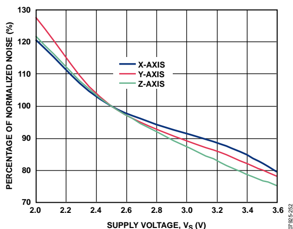
Figure 53. Normalized Noise vs. Supply Voltage, V_s
